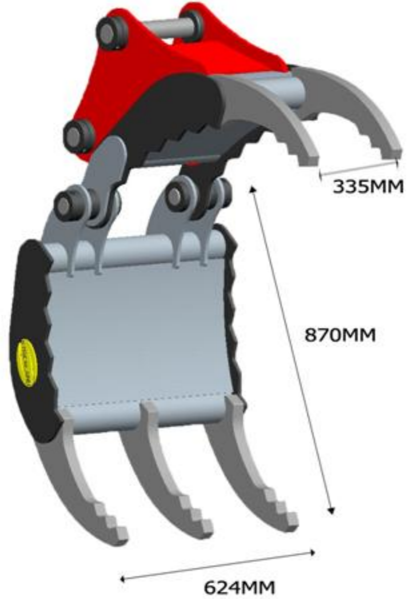
3-2 CONFIGERATION 208KG
